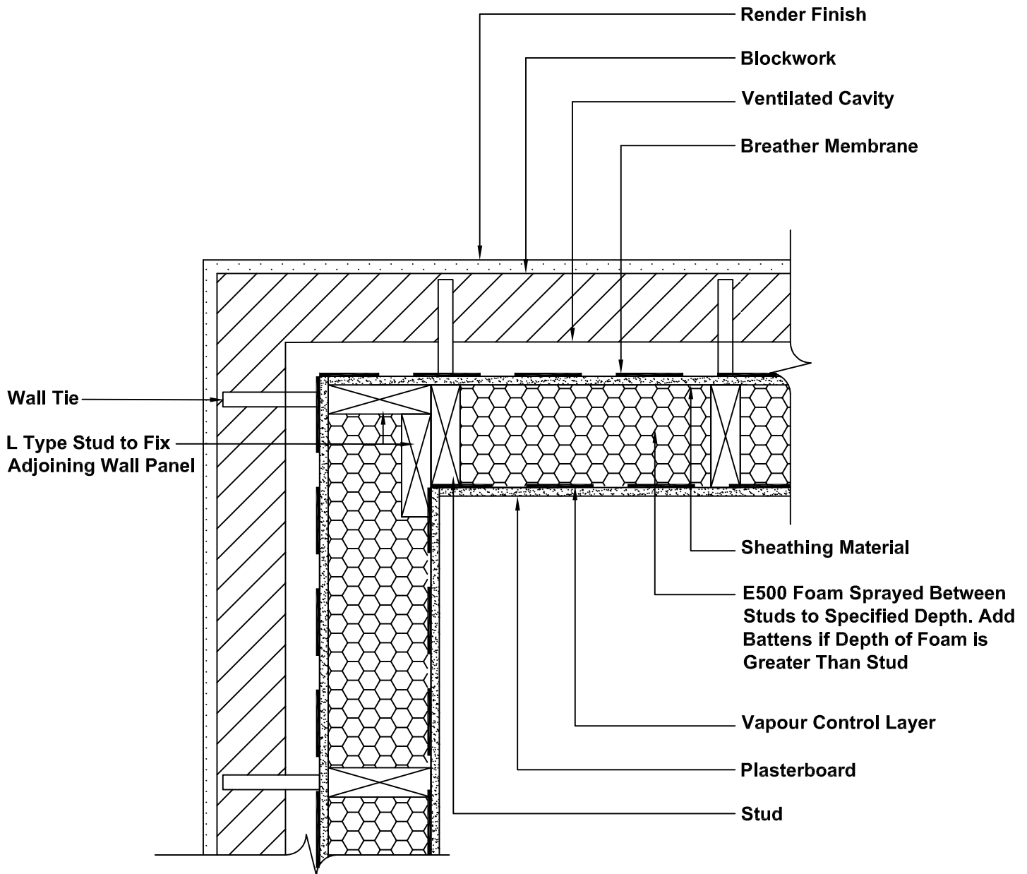
NEW BUILD TIMBER FRAME. EXTERNAL CORNER. TGD L 2008 & 2010
